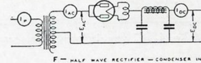
F - HALF WAVE RECTIFIER - CONDENSER INPUT
