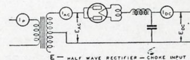
E - HALF WAVE RECTIFIER - CHOKE INPUT
