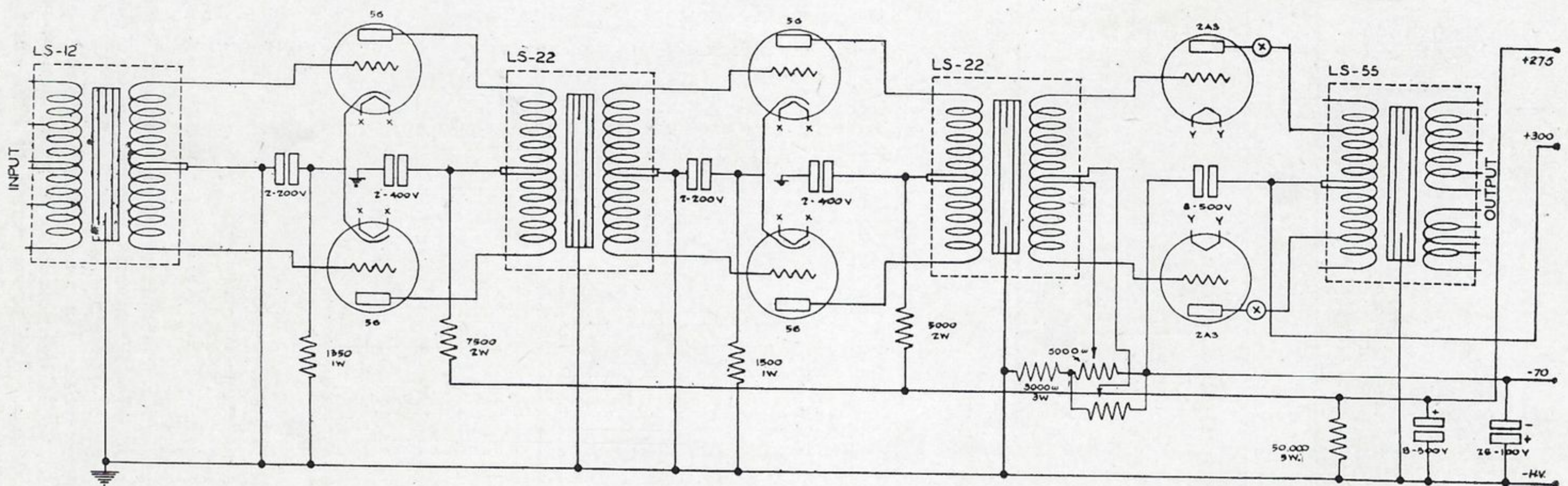
2A3 Audio Amplifier
