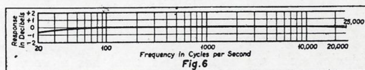
Characteristic curve of a line-matching transformer
