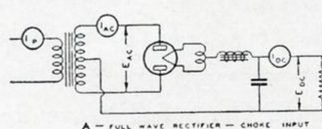
A - FULL WAVE RECTIFIER - CHOKE INPUT
