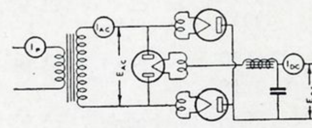
C - BRIDGE RECTIFIER - CHOKE INPUT
