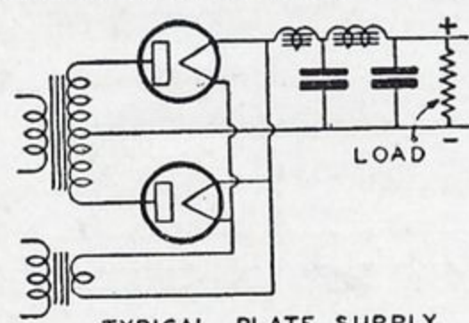
TYPICAL PLATE SUPPLY (Figure 10)
