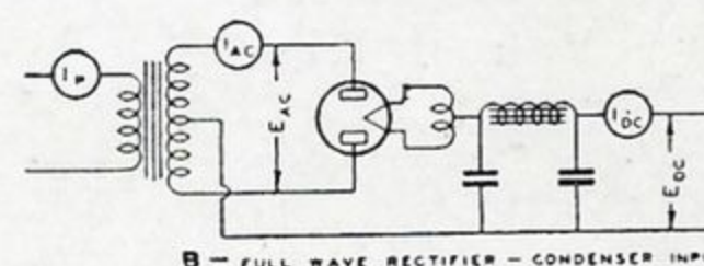
B - FULL WAVE RECTIFIER - CONDENSER INPUT
