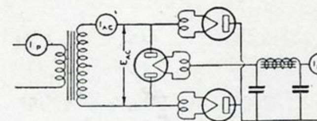
D - BRIDGE RECTIFIER - CONDENSER INPUT
